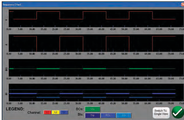
Figure 11. State Sequence Preview Screen
